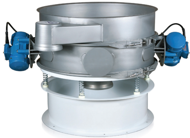
Centre Discharge Separators are available in the following diameters: 24", 30", 36", 40", 48" and 60".
